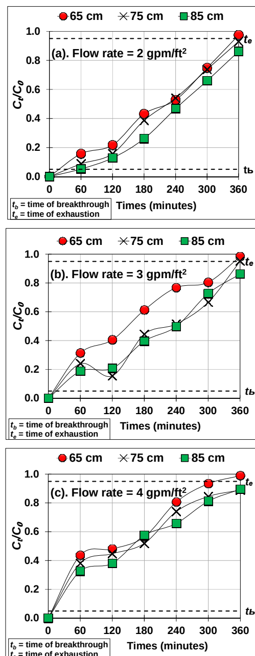
Fig. 3. Effect of various bed depth on the breakthrough curve of aluminum adsorption onto natural pumice at various flow rates: (a). 2 gpm/ft 2 , (b). 3 gpm/ft 2 and (c). 4 gpm/ft 2 (aluminum concentration = 1.14 mg/L; pH 6.2).
