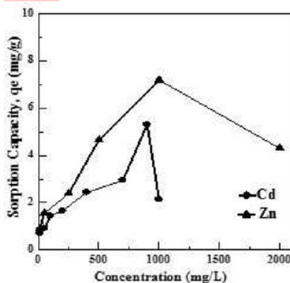
Fig. 3. Effect of concentration on the sorption capacity of Cd and Zn ions on Tanjung fruit husk. Experimental condition: pH solution of Cd = 5, pH solution of Zn = 6, biosorbent mass = 0.1 g, stirring speed = 200 rpm, contact time = 15 min, and particle size = 160 \mu m
