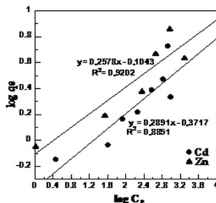
Fig. 7. Freundlich isotherm model for Cd and Zn ions biosorption on Tanjung fruit husk
