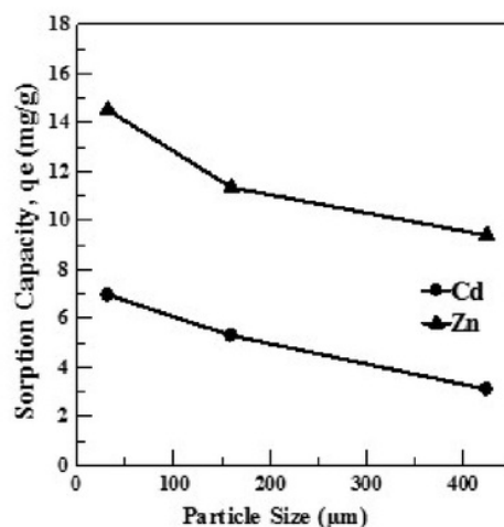
Fig. 6. Effect of particle size on the sorption capacity of Cd and Zn ions on Tanjung fruit husk. Experimental condition: pH solution of Cd = 5, pH solution of Zn = 6, Cd ion concentration = 900 mg/L, Zn ion concentration = 1000 mg/L, contact time of Cd = 15 min, contact time of Zn = 30 min, biosorbent mass = 0.1 g, and stirring speed = 200 rpm
