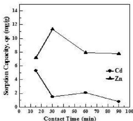
Fig. 4. Effect of contact time on the sorption capacity of Cd and Zn ions on Tanjung fruit husk. Experimental condition: pH solution of Cd = 5, pH solution of Zn = 6, Cd ion concentration = 900 mg/L, Zn ion concentration = 1000 mg/L, biosorbent mass = 0.1 g, stirring speed = 200 rpm, and particle size = 160 \mu m
