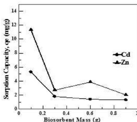
Fig. 5. Effect of biosorbent mass on the sorption capacity of Cd and Zn ions on Tanjung fruit husk. Experimental condition: pH solution of Cd = 5, pH solution of Zn = 6, Cd ion concentration = 900 mg/L, Zn ion concentration = 1000 mg/L, contact time of Cd = 15 min, contact time of Zn = 30 min, stirring speed = 200 rpm, and particle size = 160 \mu m
