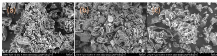
Fig. 10. Scanning electron microscope husk of Mimosa elengi L. before sorption (a), after Zn ion sorption, and after Cd ion sorption (c). Magnification 500 times
