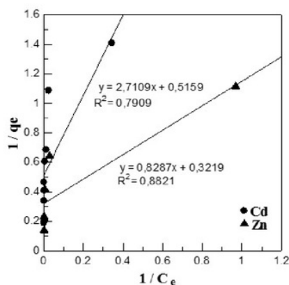
Fig. 8. Langmuir isotherm model for Cd and Zn ions biosorption on Tanjung fruit husk
