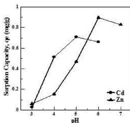
Fig. 2. Effect of pH on Zn and Cd ion biosorption by on Tanjung fruit husk. Experimental condition: concentration = 10 mg/L, biosorbent mass = 0.1 g, stirring speed = 200 rpm, contact time = 15 min, and particle size = 160 \mu m
