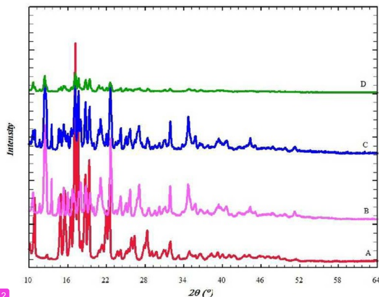
Figure 4. Powder X-ray diffraction pattern of (A) simvastatin, (B) \beta -cyclodextrin, (C) physical mixture of simvastatin with \beta -cyclodextrin, and (D) inclusion complexes of simvastatin with \beta -cyclodextrin
