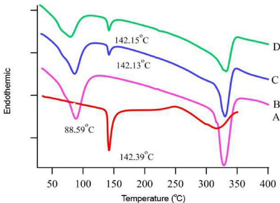
Figure 3. Differential thermal analysis thermogram of (A) simvastatin, (B) \beta -cyclodextrin, (C) physical mixture of simvastatin with \beta -cyclodextrin, and (D) inclusion complexes of simvastatin with \beta -cyclodextrin
