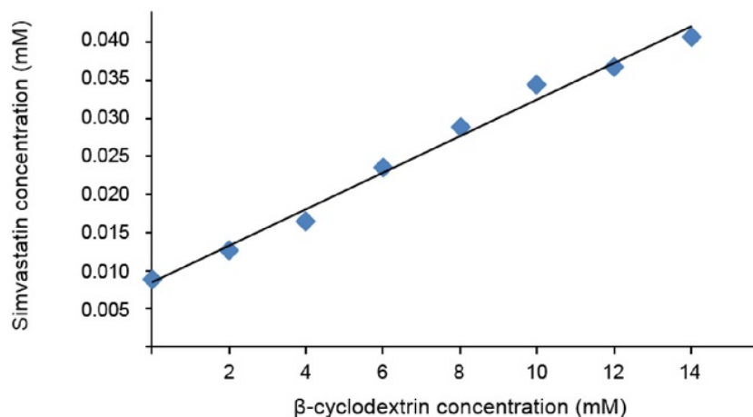
Figure 1. Phase solubility diagram of simvastatin with \beta -cyclodextrin in water at room temperature
