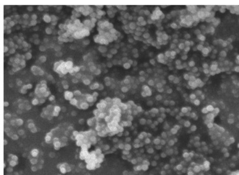
Figure 4: The image of verapamil hydrochloride microcapsules surface detected using SEM at magnification of 2,500 times.
