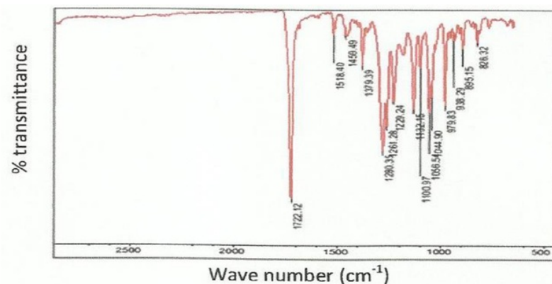
Figure 3: FTIR spectrum of verapamil hydrochloride microcapsules.
