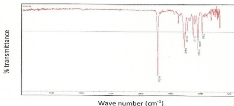
Figure 2: FTIR spectrum of P(3HB).
