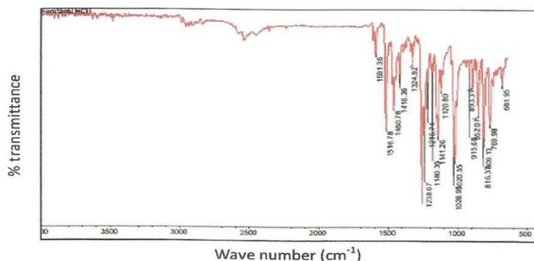
Figure 1: FTIR spectrum of verapamil hydrochloride.
