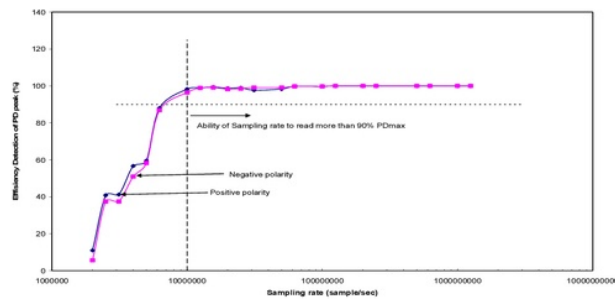
Figure 6. Detection efficiency of PD number per phase function of sampling rate
