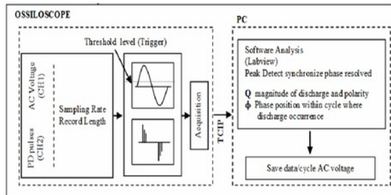
Figure 3. Analog to digital PD waveform synchronization process
