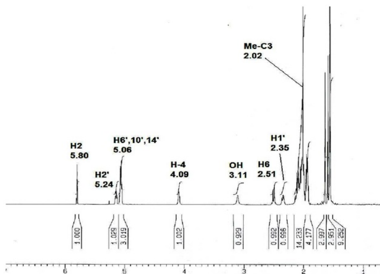
Fig. 3: ^1H -NMR spectrum of TPTQ in CDCl_3
