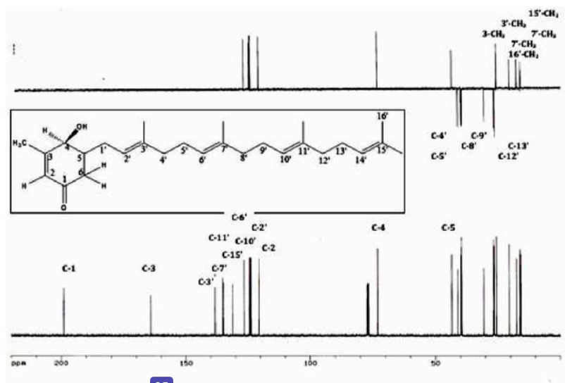
35 Fig. 2: ^{13}C -NMR and DEPT spectra of TPTQ in CDCl_3
