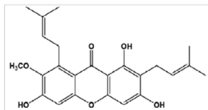
Fig. 1: Structure of \alpha -mangostin
