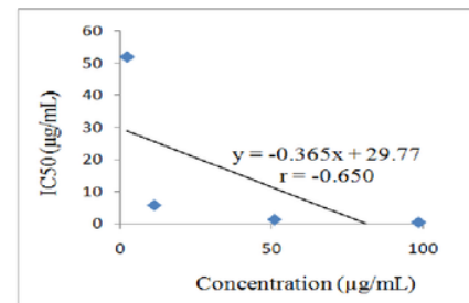
Fig. 6: Correlation between \alpha -mangostin concentration and IC 50
