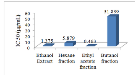
Fig. 5: IC 50 value of ethanol extract and fractions of G. mangostana L. against T47D cell line
