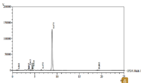
Fig. 2: Chromatogram of the standard α-mangostin. System suitability parameters were within the acceptance limits, ideal for the chromatographed sample
