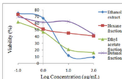
Fig. 4: Viability (%) of T47D cells in different concentrations of G. mangostana L.
