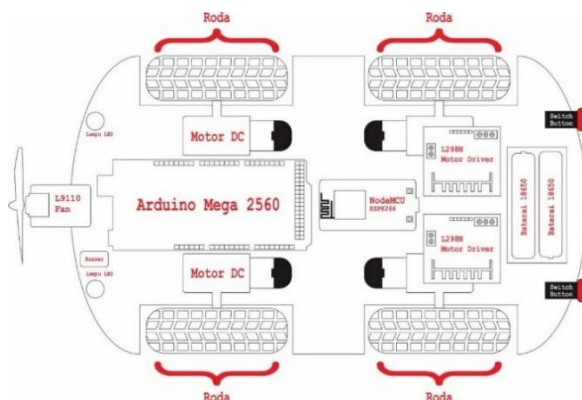
Figure 3. Hardware Design
