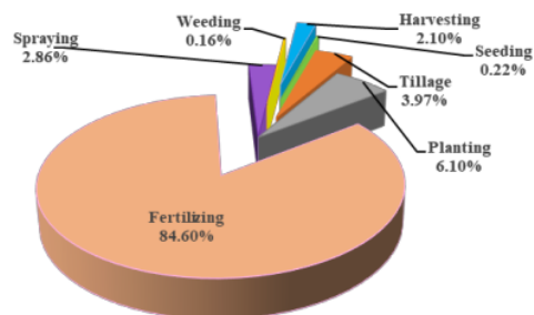
Figure 8. Percentage of energy in each operating activity
