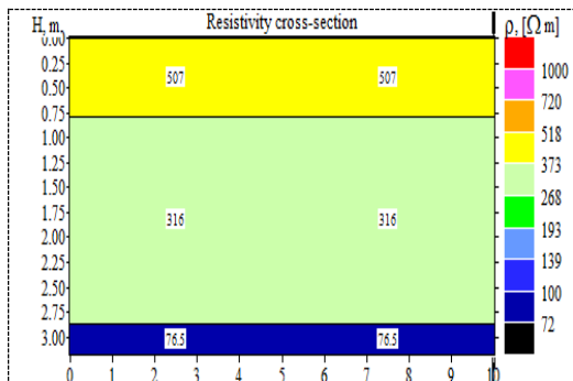
Figure 11. Geoelectrical section point 9
