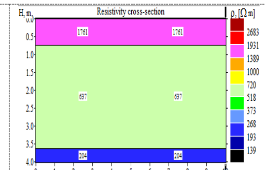
Figure 12. Geoelectrical section point 10
