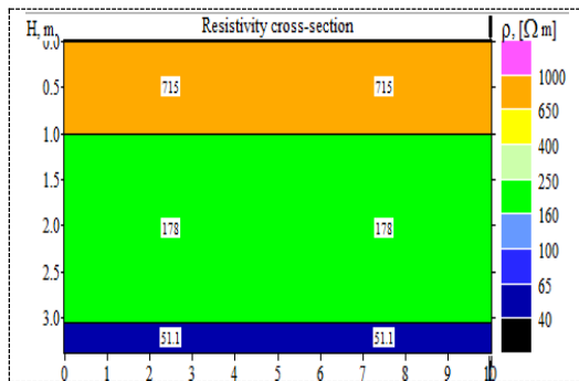
Figure 7. Geoelectrical section point 5
