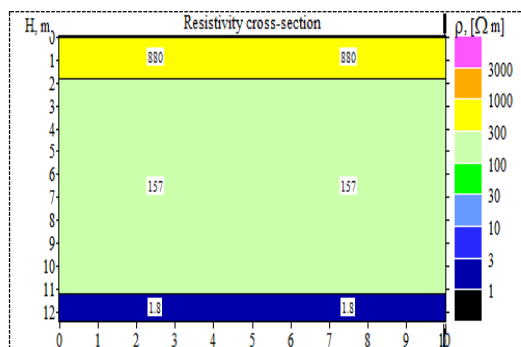
Figure 9. Geoelectrical section point 7
