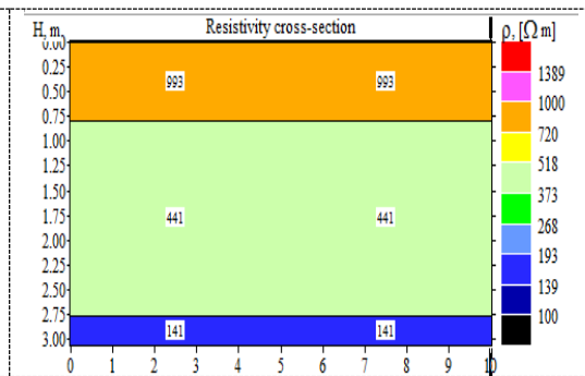
Figure 8. Geoelectrical section point 6
