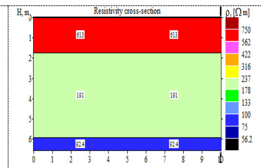
Figure 10. Geoelectrical section point 8
