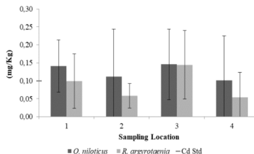
Figure 5. Concentration of Cd Metal in Rasbora argyrotaenia and Oreochromis niloticus . 1. Dense Settlement; 2. Hydropower; 3. Fish Cage; 4. Endemic Fisheries. Cd Std: Standard of Cd in fish
