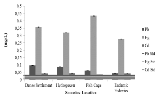
Figure 2. Heavy metals concentration in Maninjau Lake waters
