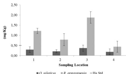
Figure 4. The concentration of Hg Metal in Rasbora argyrotaenia and Oreochromis niloticus . 1. Dense Settlement; 2. Hydropower; 3. Fish Cage; 4. Endemic Fisheries. Hg Std: Standard of Hg in Fish
