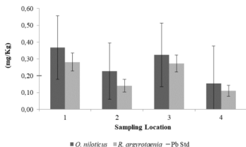
Figure 3. The concentration of Pb Metal in Rasbora argyrotaenia and Oreochromis niloticus . Note: 1. Dense Settlement; 2. Hydropower; 3. Fish Cage; 4. Endemic Fisheries. Pb Std: Standard of Pb in fish
