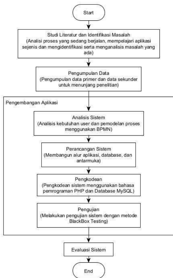
Gambar 2. Flowchart penelitian
