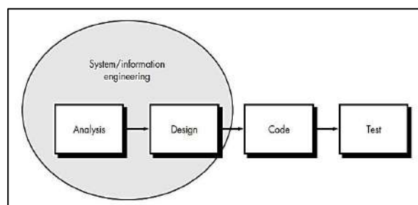
Gambar 1. Metode waterfall
