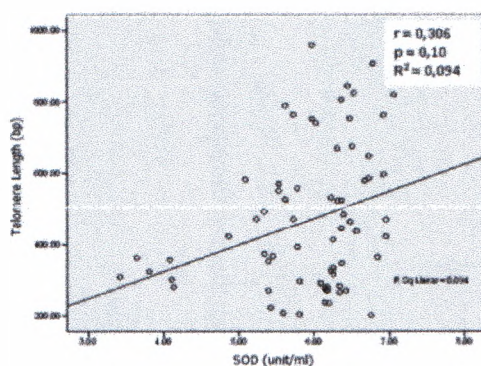
Figure 2: Correlation between SOD and telomere length of Minangkabau ethnic men.
