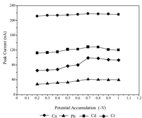
Fig. 5. The potential accumulation relationship curve to the peak current ( I_p ) of the metal ion simultaneously, condition: 10 mL mixture of 10 µg/L; 0.2 mL of fluorexon 0.6 mM; 0.2 mL KCl 0.1 M; time accumulation 60 s; pH 6
