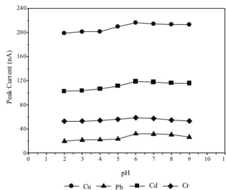
Fig. 4. The curve of pH relationship to the peak current ( I_p ) of metal ions simultaneously, conditions: 10 mL mixture 10 \mu\text{g/L} ; 0.2 mL of fluorexon 0.6 mM; 0.2 mL KCl 0.1 M; time 60 s; potential accumulation -0.7 V
