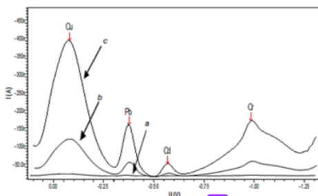
39 Fig. 2. Adsorptive stripping voltammetry scan of Cu, Pb, Cd and Cr in the presence of fluorexon. 10 mL Mixture 10 µg/L; 0.2 mL of fluorexon 0.6 mM; 0.2 mL KCl 0.1 M; potential accumulation of -0.7 V; time accumulation 70s; pH 6
