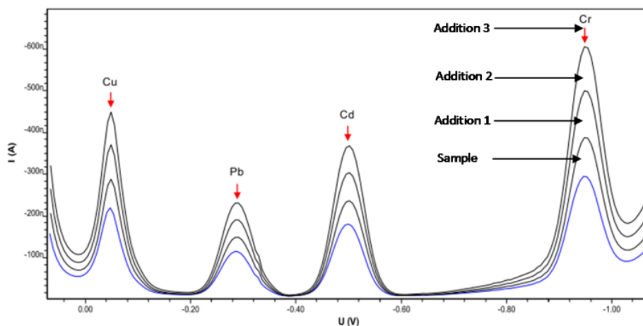
Fig. 8. Voltammogram of Cu, Pb, Cd, and Cr in Tap water sample in the presence of 0.2 mL of fluorexon 0.6 mM; 0.2 mL KCl 0.1 M; deposition potential of -700 mV; deposition time 70 s; pH 6
