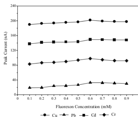
Fig. 3. The relation curve of fluorexon concentration to the peak current ( I_p ) ion metals simultaneously, conditions: 10 mL of standard solution mixed 10 \mu\text{g/L} 0.2 mL fluorexon; KCl 0.1 M; time 60 s; potential -0.7 V; pH 6
