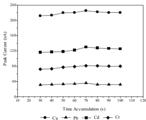
Fig. 6. The time accumulation relationship curve to the peak current ( I_p ) of metal ions simultaneously, condition: 10 mL Mixture 10 \mu\text{g/L} ; 0.2 mL of fluorexon 0.6 mM; 0.2 mL KCl 0.1 M; potential accumulation of -0.7 V; pH 6
