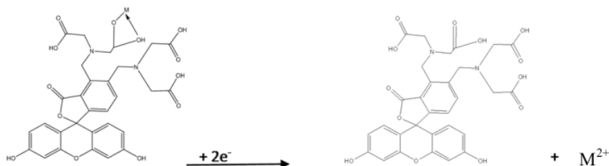
Fig .1. Mechanism of the electrochemical reduction process for complex Fluorexon-metal complex
