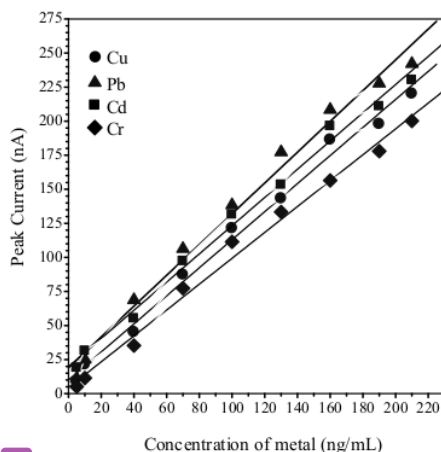
Fig. 7. Calibration graph for (Cu, Pb, Cd and Cr) in the presence of 0.2 mL of fluorexon 0.6 mM; 0.2 mL KCl 0.1 M; potential accumulation of -0.7 V; time accumulation 70 s; pH 6
