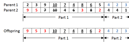
Figure 6. Illustration of the crossover process [5]
