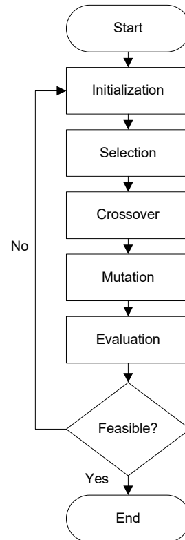
Figure 3. General structure of GA [4]
