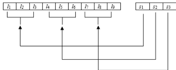
Figure 5. Example of a two-part chromosome [5]
