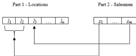
Figure 4. Structure of the two-part chromosome [5]
