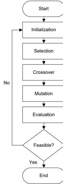
Figure 3. General structure of GA [4]
