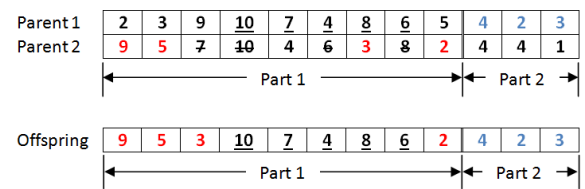
Figure 6. Illustration of the crossover process [5]
