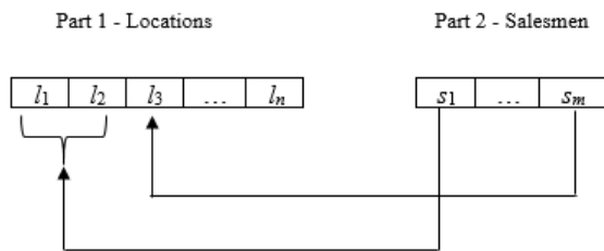
Figure 4. Structure of the two-part chromosome [5]
