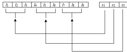
Figure 5. Example of a two-part chromosome [5]
