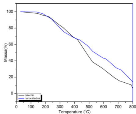
Figure 3. TGA curves the extracted catechin and nanocatechin
