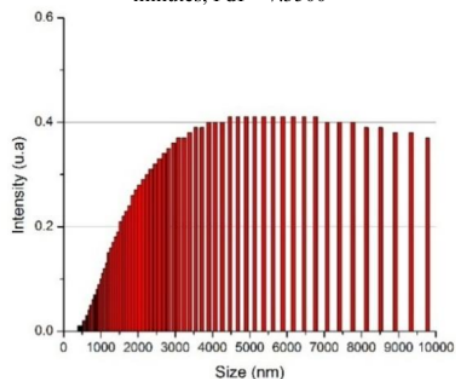
(c) Particle distribution with homogenization time of 45 minutes, PdI = 3.9130
