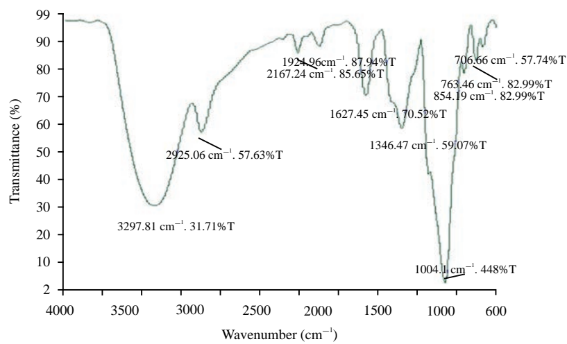
Fig. 3: FT-IR spectrum of banana cv. Raja starch
