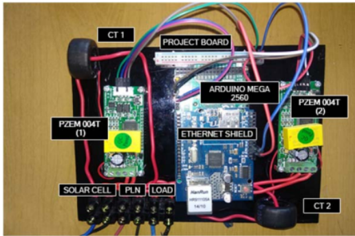
Figure 2. Web-based Net Energy Meter Real Circuit
