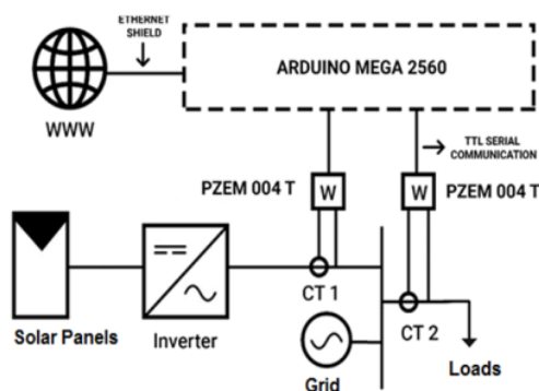
Figure 1. PZEM Based Net Energy Meter
