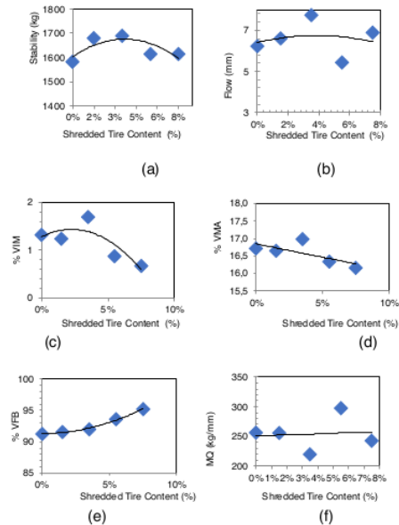
Figure 2. Marshall results for Optimum Shredded Tyre determination
