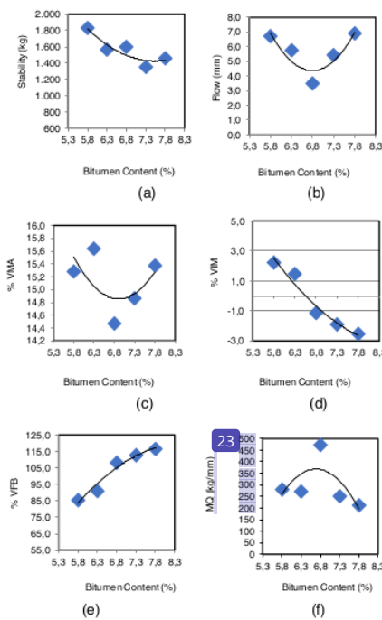
Figure 1. Marshall test results for optimum bitumen content determination
