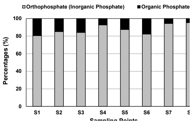
Fig. 3. Ratio of orthophosphate and organic phosphate in total phosphates concentrations at 8 sampling points.
