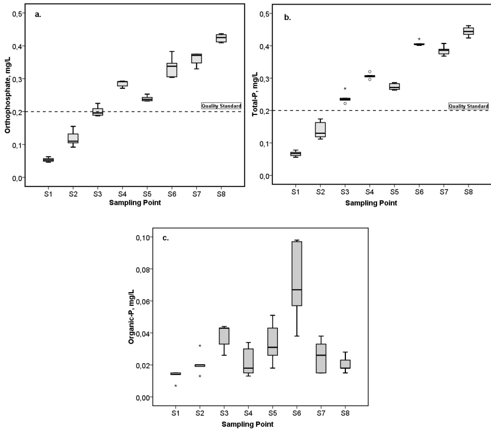
Fig. 2. Spatial variations of (a) Orthophosphate, (b) Total-P, and (c) Organic-P in Batang Arau river.
