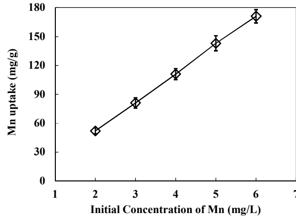
FIGURE 6. Effect of initial concentration on adsorption capacity of manganese onto pumice (adsorbent dose: 0.3 g/L; contact time: 90 min; diameter of adsorbent: <149 \mu m; pH: 4).
