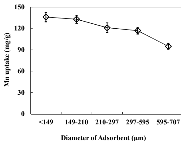
FIGURE 4. Effect of diameter of absorbent on adsorption capacity of manganese onto pumice (manganese concentration: 5 mg/L; pH: 8; adsorbent dose: 0.3 g/L; contact time; 90 min).
