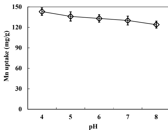
FIGURE 5. Effect of pH on adsorption capacity of manganese onto pumice (manganese concentration: 5 mg/L; adsorbent dose: 0.3 g/L; contact time: 90 min; diameter of adsorbent: <149 μm).
