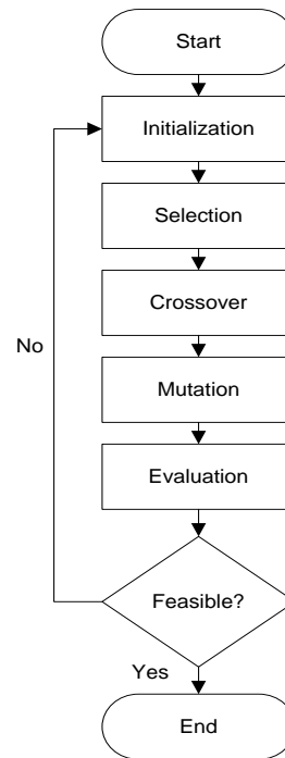
Figure 3. General structure of GA [4]
