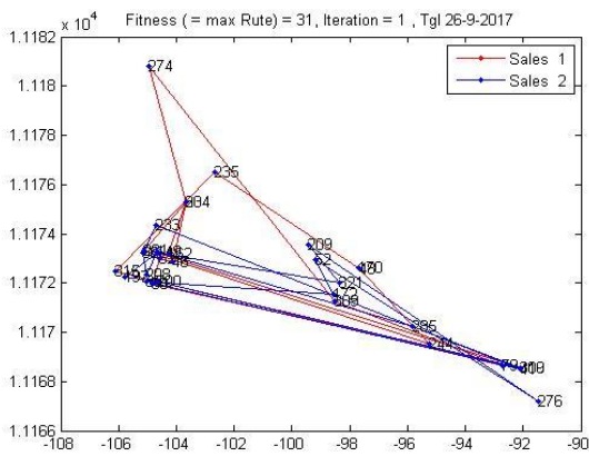
Figure 9. Animated distribution routes (2 salesmen)
