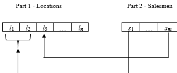
Figure 4. Structure of the two-part chromosome [5]
