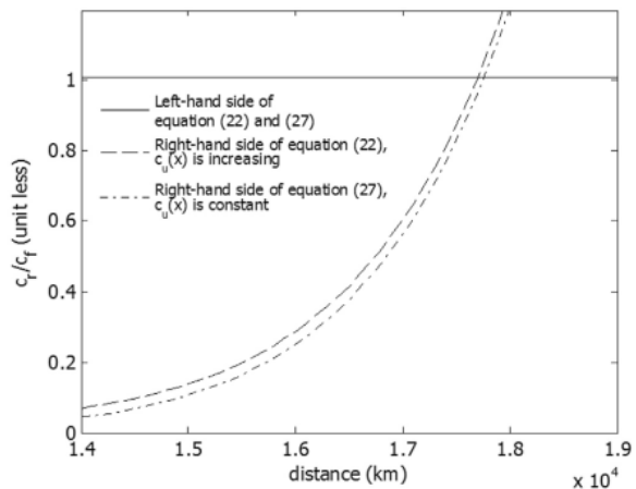
Fig. 6. The effect of c_u(x) on x_c^* .
