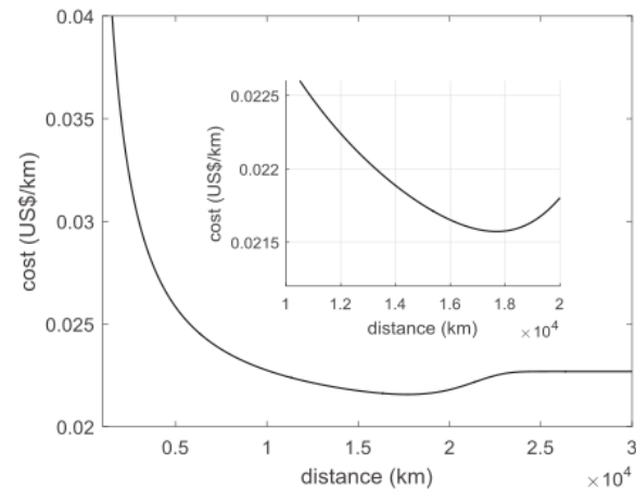
Fig. 3. Plot of cost minimization problem objective function.
