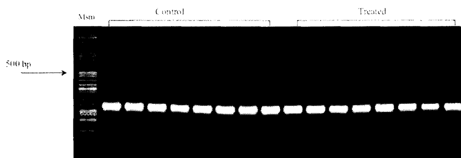
Figure 4. The electrophoresis result of PCR amplification with SRY primers. Each sample showed the good quality of DNA band. Position of band was at 500bp. Representative gels of eight samples from control and treated groups are shown. Msm = molecular size marker
