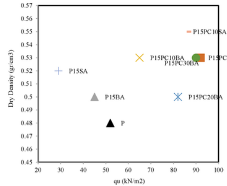
Fig. 7 Relationship Between UCS and Dry Density of Peat Soil Stabilized With BA, SA, and PC
