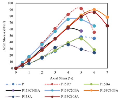
Fig. 9 Stress and Strain Relationship for Peat Soils Stabilized with PC, BA, and SA.
