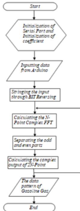
10 Figure 2. The flow diagram of the main program of the FFT algorithm
