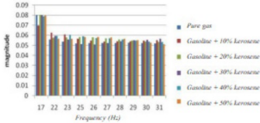
Figure 5. FFT Spectrum of Gasoline Sample
