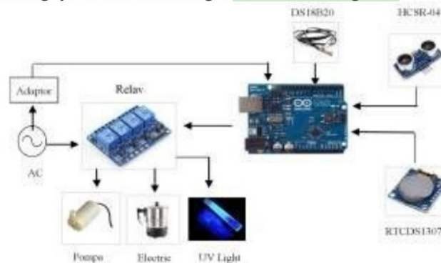
Figure 3. The design of the hardware system
