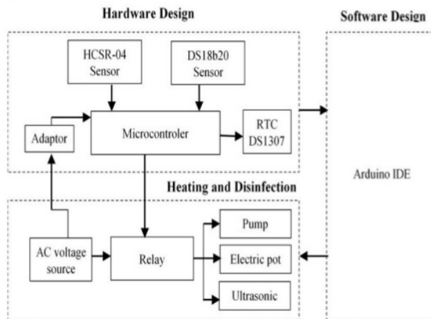
Figure 2. Block design process system
