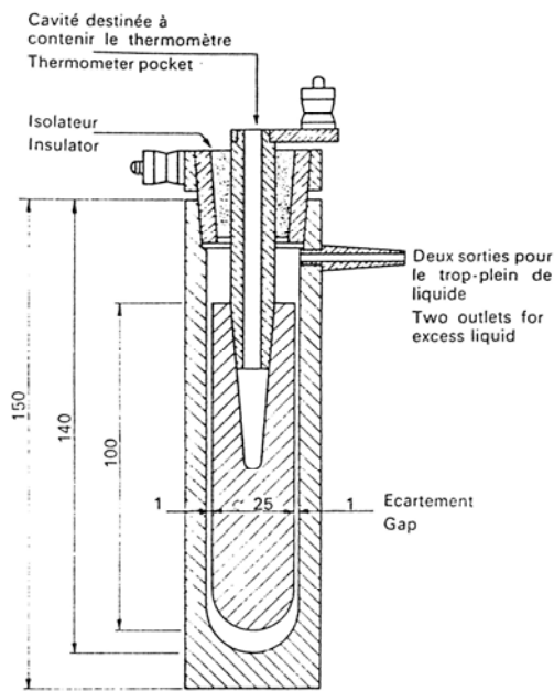
Gambar 3 Test Cell dua terminal [10]
