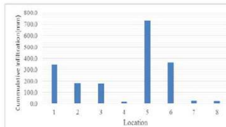
Fig 9 Correlation of cumulative infiltration with the research location in the downstream watershed in Padang.
