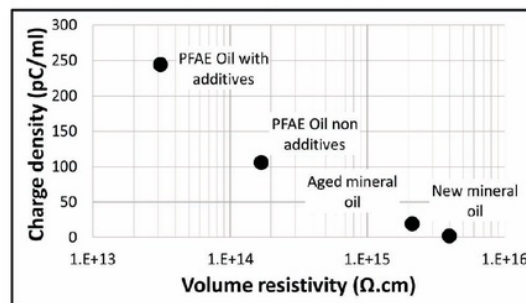
Fig.8. Relationship between charge tendency and volume resistivity
