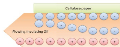
Fig.3. Charge separation at pressboard duct of power transformer due to friction
