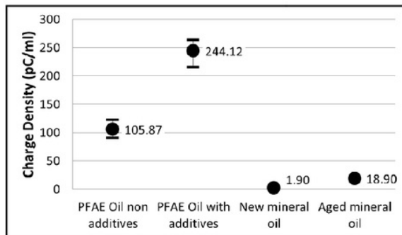
Fig.5. ECT on several sample oil
