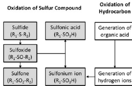
Fig.6. Mechanism of increasing ECT in mineral oil due to sulfur compound [5]
