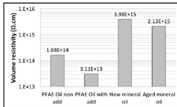
Fig.7. Volume resistivity on each type of oil
