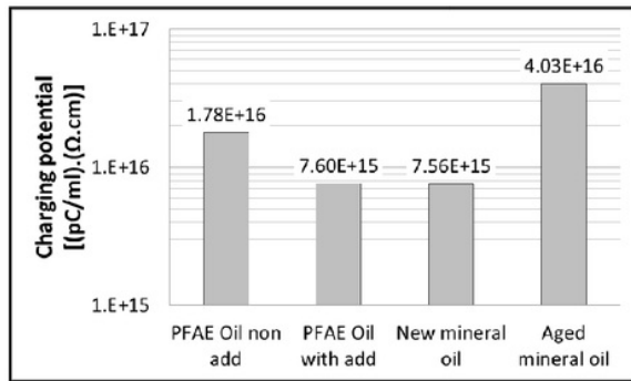
Fig.9. Charging potential on each type of oil
