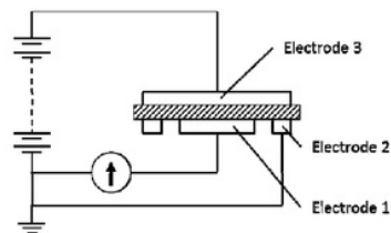
Fig.4. Basic connection for guarded electrodes
