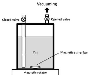
Fig.1. Preconditioning system
