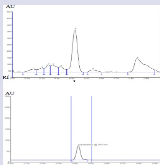
Figure 2: HPTLC chromatogram sample G. cowa R. extracts and standard rubraxanthone.
