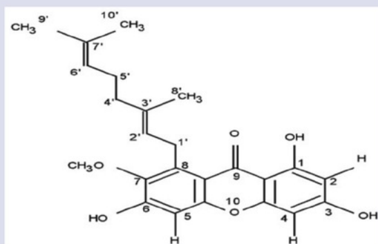
Figure 1: Structure of Rubraxanthone. 2
