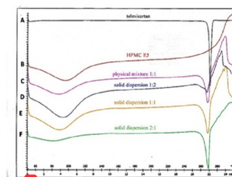
Fig. 4: Thermogram DSC of (A) TMS, (B) HPMC E5 LV, (C) Physical Mixture, (D) Solid Dispersion 1:2, (E) Solid Dispersion 1:1, and (F) Solid Dispersion 2:1
