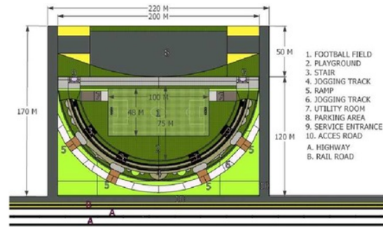
Fig. 7 Site's Functional of Proposed Man-made Hill
