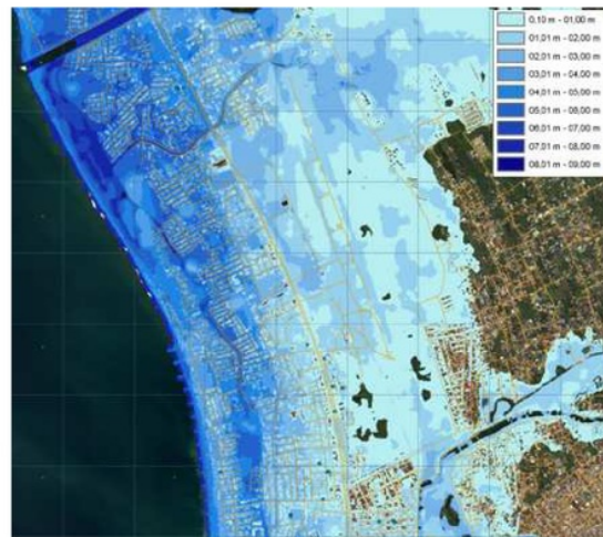
Fig. 5 Tsunami Inundation Area (Source: https://gempapadang.wordpress.com )
