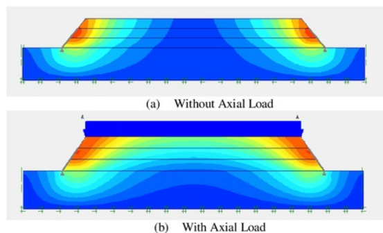
Fig. 9 Numerical Results of Slope Stability Analysis
