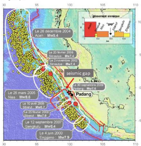
Fig. 1 The Sumatran Seismic Crisis [5]
