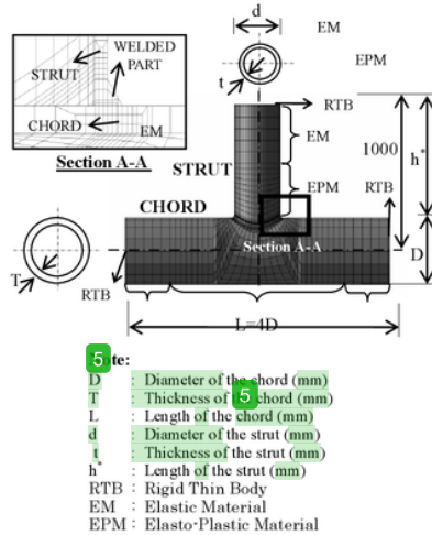
Figure.2 Numerical Model of T-Joint
