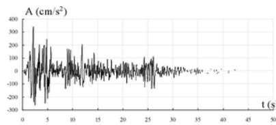
Figure. 4 Time history of El-CentroNS
