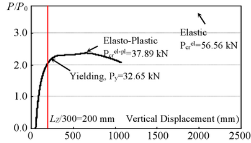
Figure.4 Static Response of Loading-Displacement
