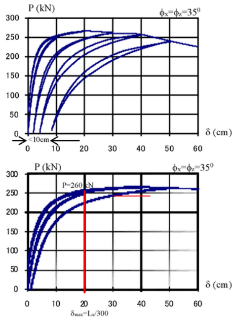
Figure.5 Static Responses of Roof Structure under Repeated Loading: (a) at the critical joint (top) (b) at the maximum vertical deflection joint (below)
