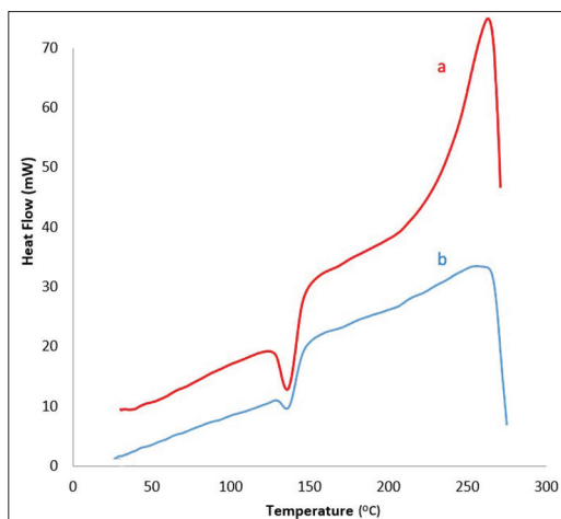
Figure 4: Thermogram of (a) intact efavirenz, (b) milled efavirenz
